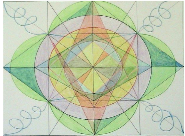
Above: A 5D energy diagram for the Earth
