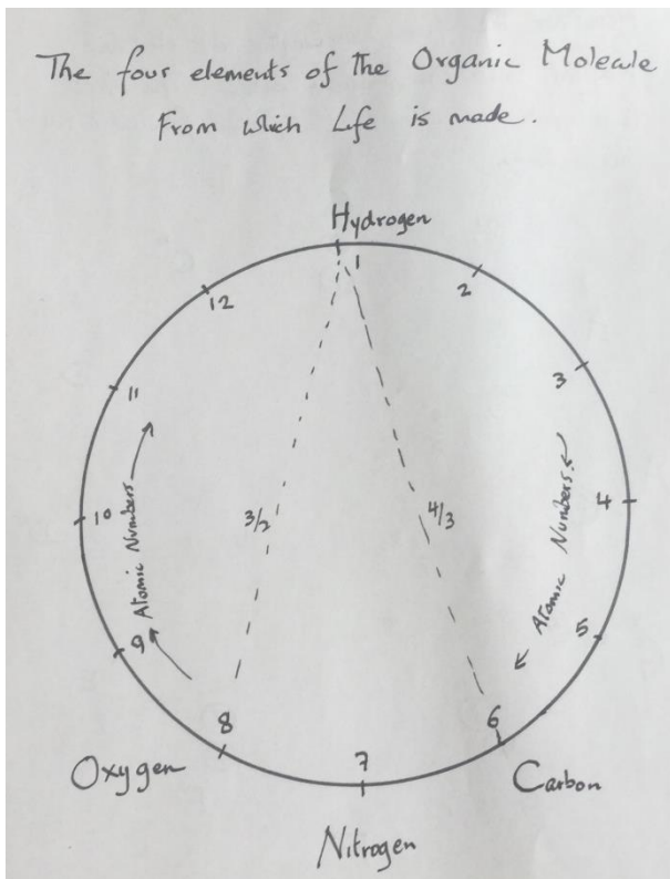
Above: The alignment of the Organic Molecule
