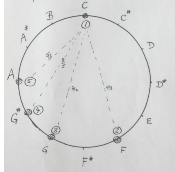
Above: The 5 Electron Wavelengths for Hydrogen Mapped to Musical Notes
